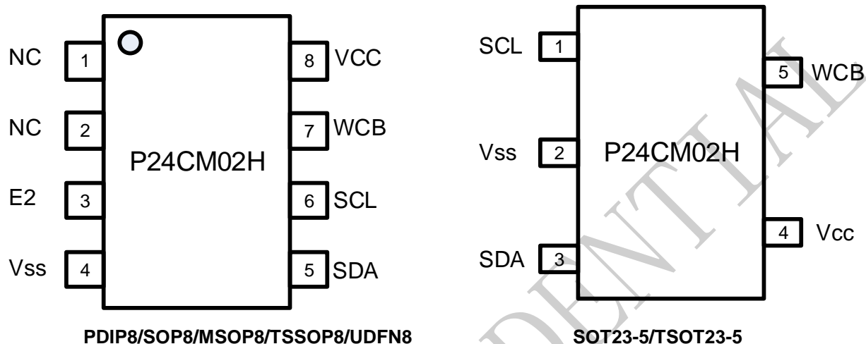
Figure 1-1 Pin Configuration
